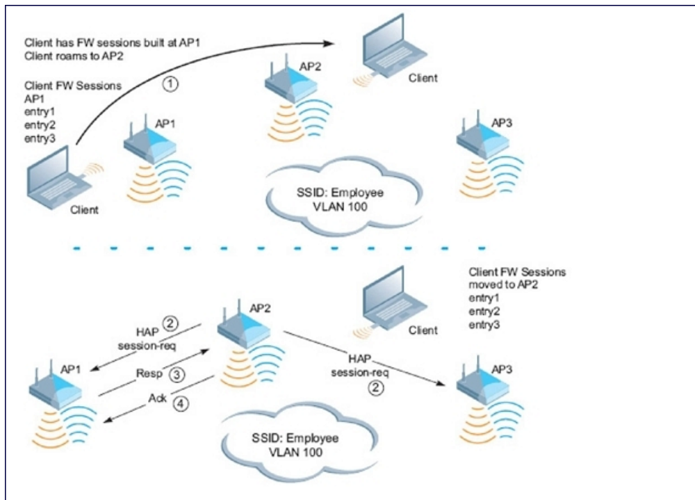
Figure 96 Bridge Mode Mobility
