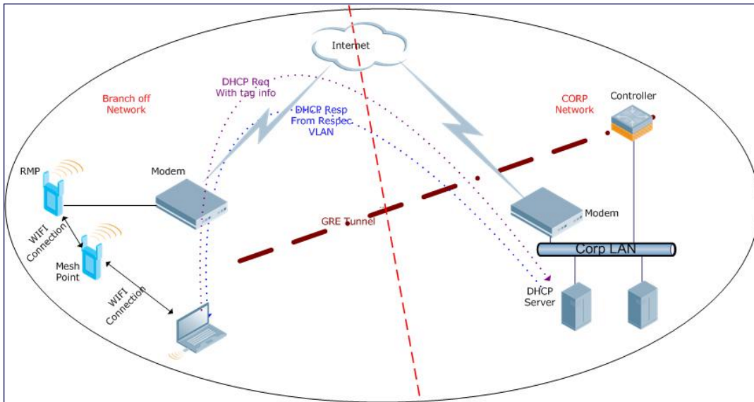
Figure 85 Working of Remote Mesh Portal
