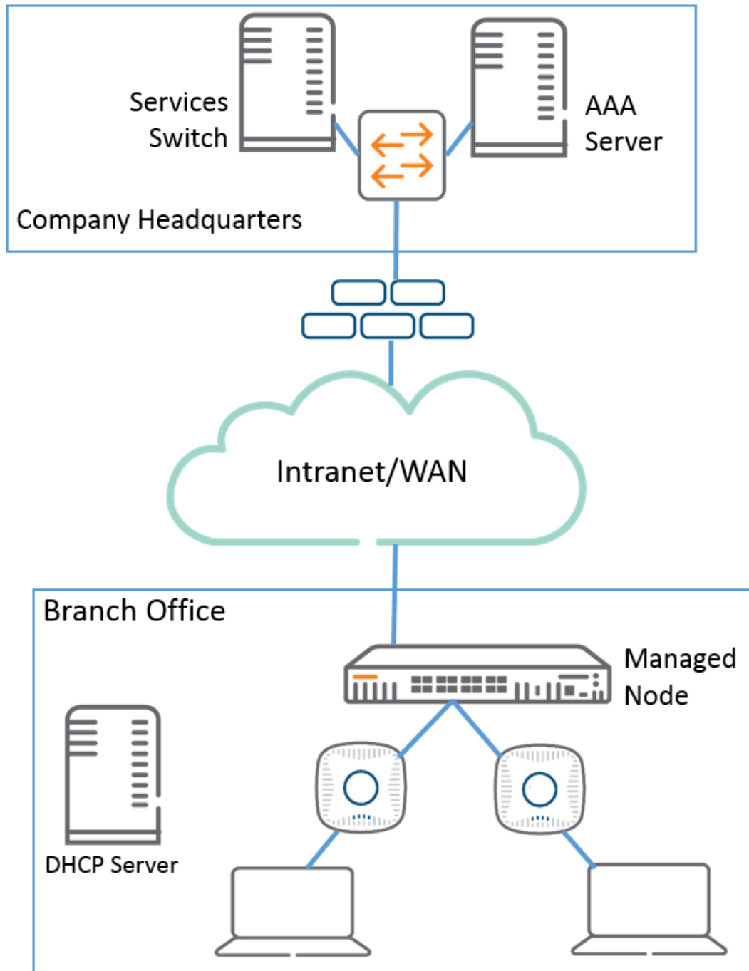
Figure 27 Managed Device Topology
