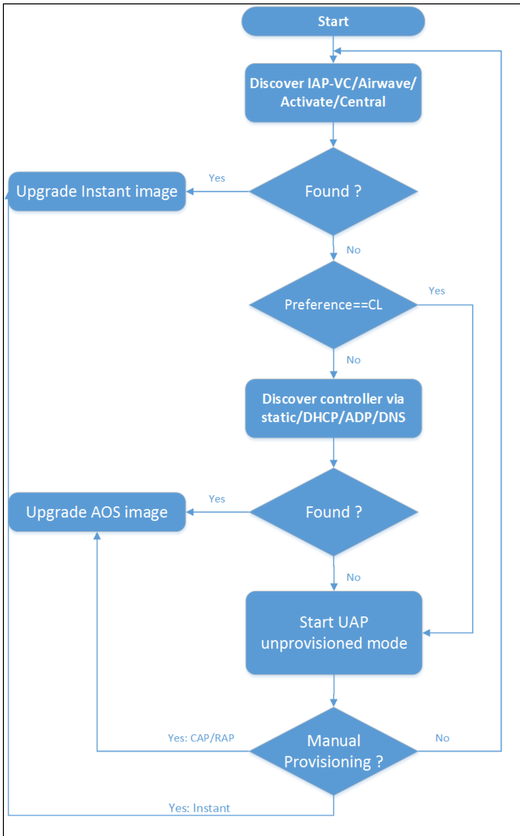
Figure 82 AP Discovery Logic
