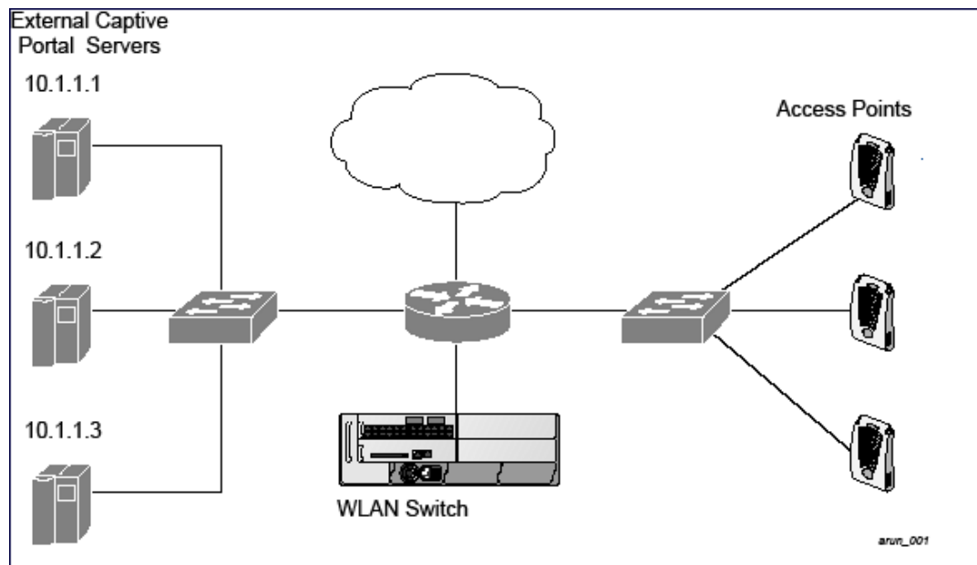
Figure 128 Example NAT-Mode Topology
