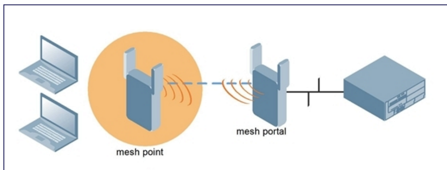
Figure 86 Sample Wireless Backhaul Deployment
