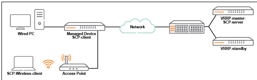
Figure 116 Sample Topology - VRRP Master as SCP Server
