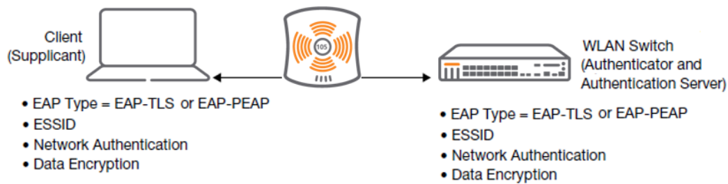
Figure 32 802.1X Authentication with Termination on Managed device
