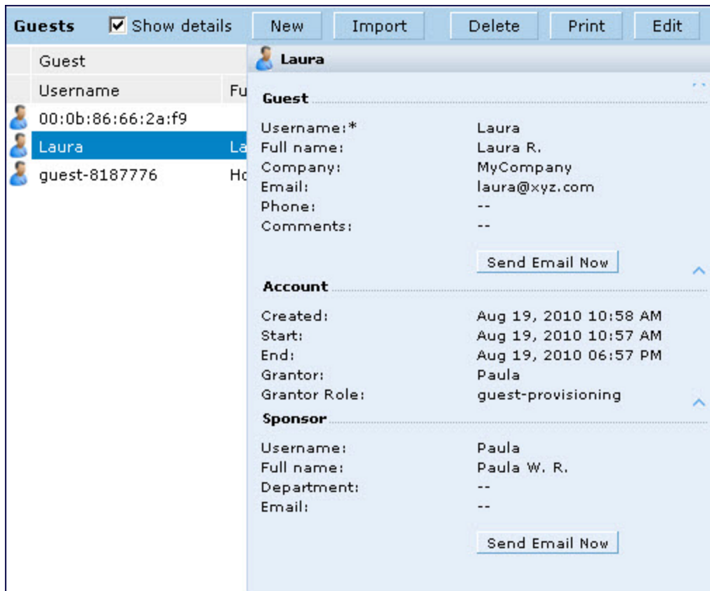
Figure 109 Creating a Guest Account—Show Details Pop-up Window
