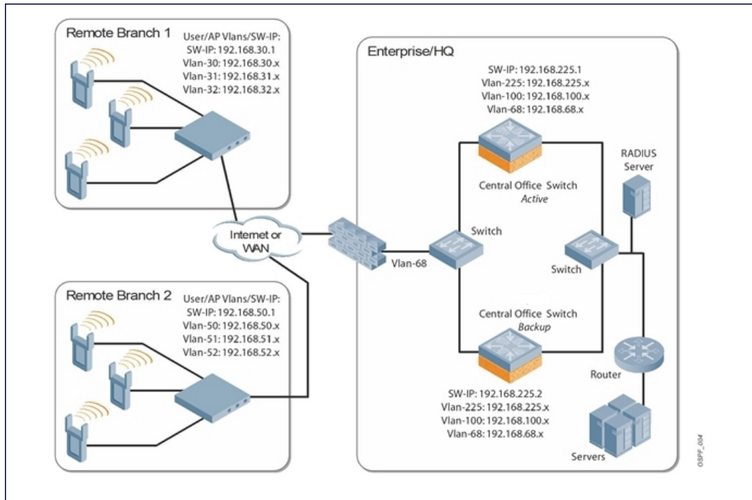
Figure 18 Sample OSPF Topology
