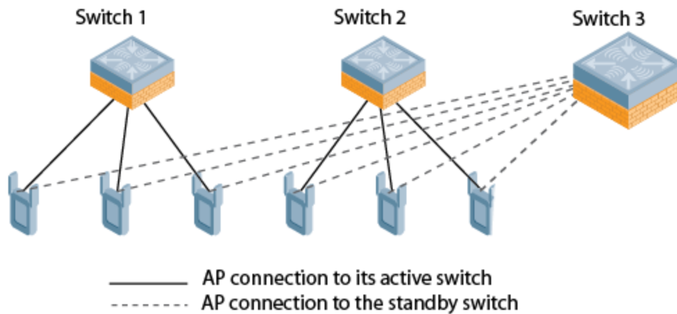
Figure 92 1:1 Active/Standby Deployment
