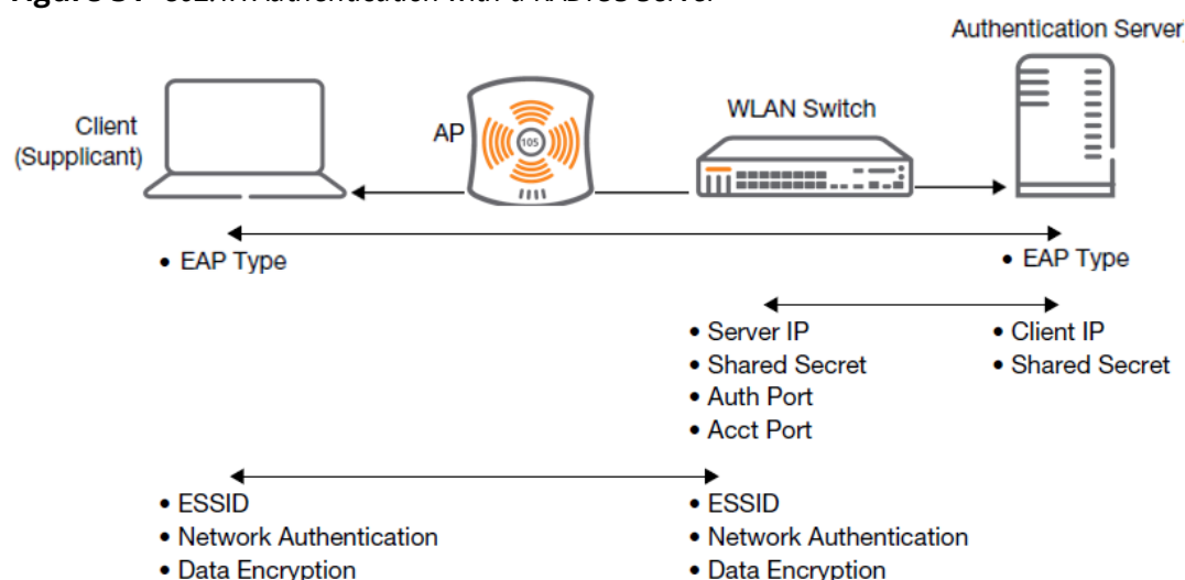
Figure 31 802.1X Authentication with a RADIUS Server
