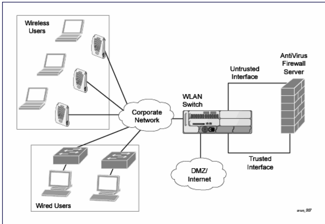
Figure 122 ESI-Fortinet Topology
