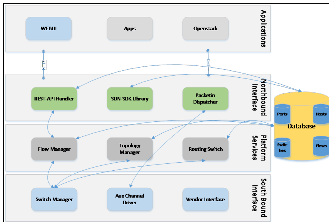
Figure 117 SDN Switch Architecture
